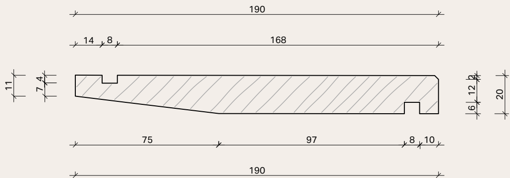
SUGi Japanese Cedar ST62 190x20mm Bevel Back Weatherboard
