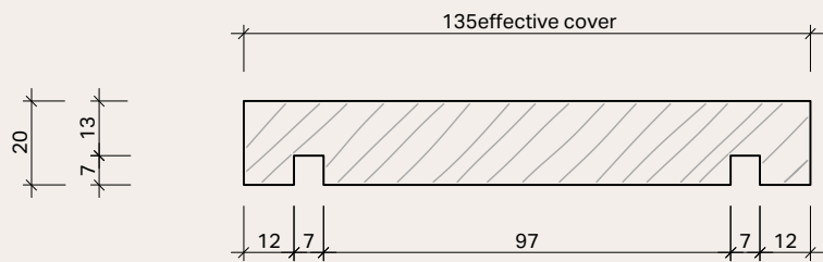
SUGi Japanese Cedar ST69 135X20mm Fascia
