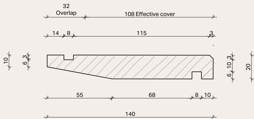
SUGi Japanese Cedar ST61 140x20mm Bevel Back Weatherboard
