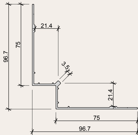
VTFL - 39 Internal corner flashing 19mm
