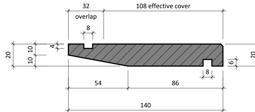
ST61 Horizontal Bevel Back Weatherboard
